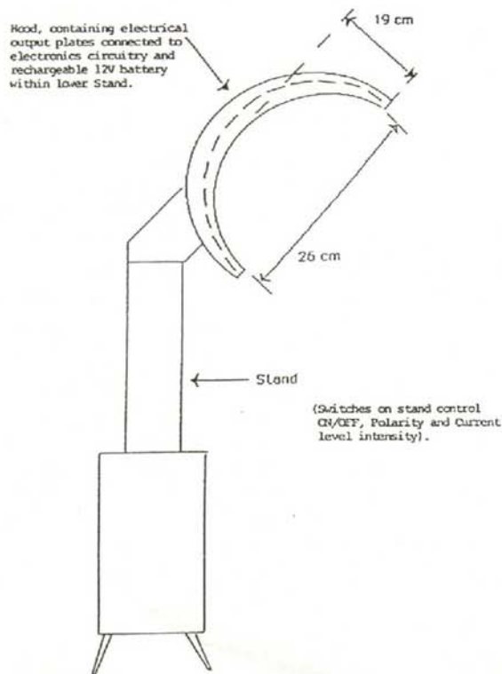
FIG. 1. Hair regrowth device.
